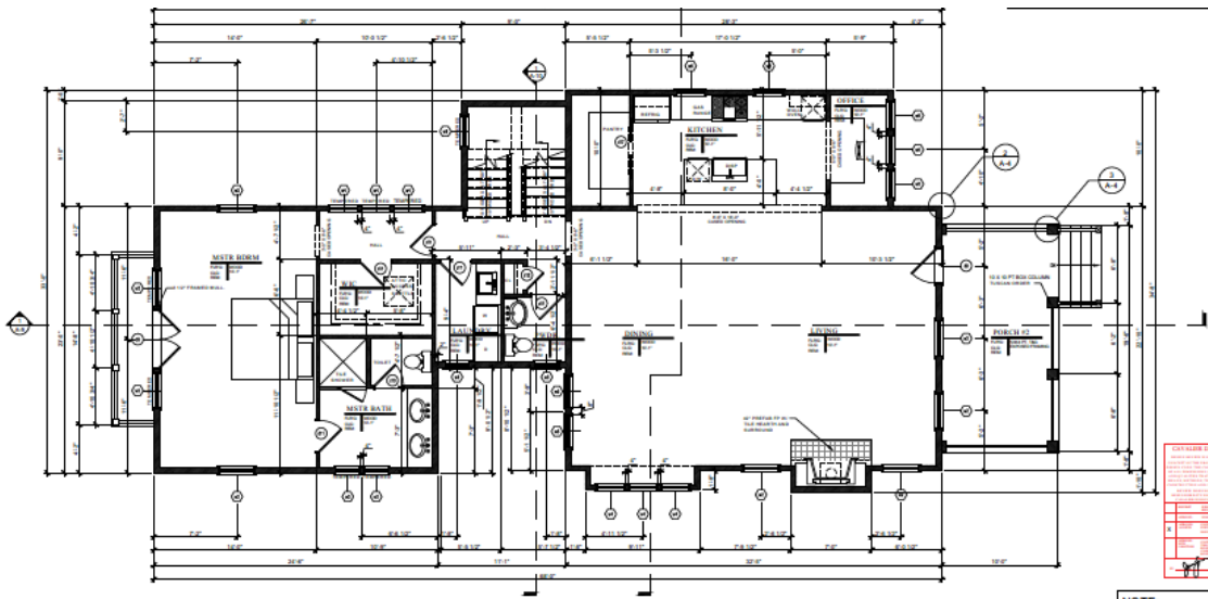
A FIRST FLOOR PLAN 1/4" = 1'-0"
