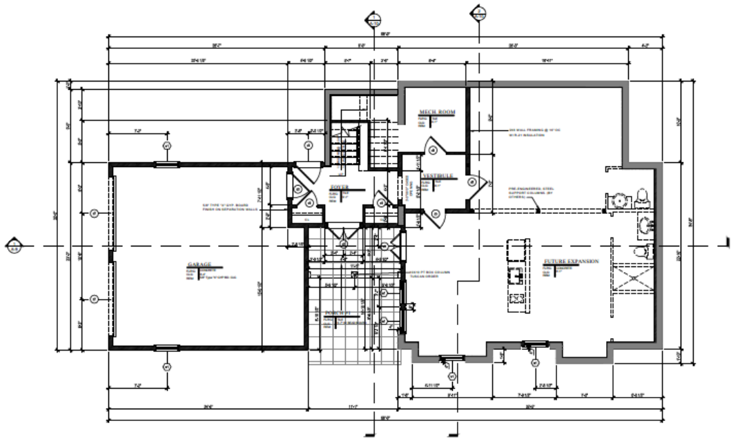
B BASEMENT FLOOR PLAN 1/4" = 1'-0"
